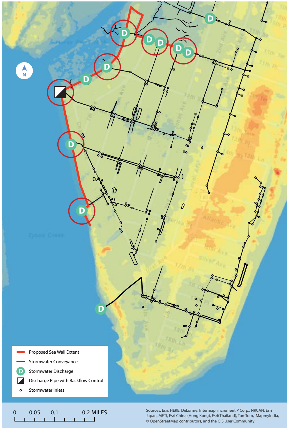
FIGURE 4.10: VISUALIZATION OF STORMWATER BACKFLOW AND SEA WALL ACTIONS FOR CITY OF TYBEE ISLAND, SOUTHWEST QUADRANT. RED CIRCLES INDICATE DISCHARGE POINTS THAT SHOW CONNECTIVITY TO LOW-LYING AREAS VULNERABLE TO TIDAL BACKFLOW FLOODING.
