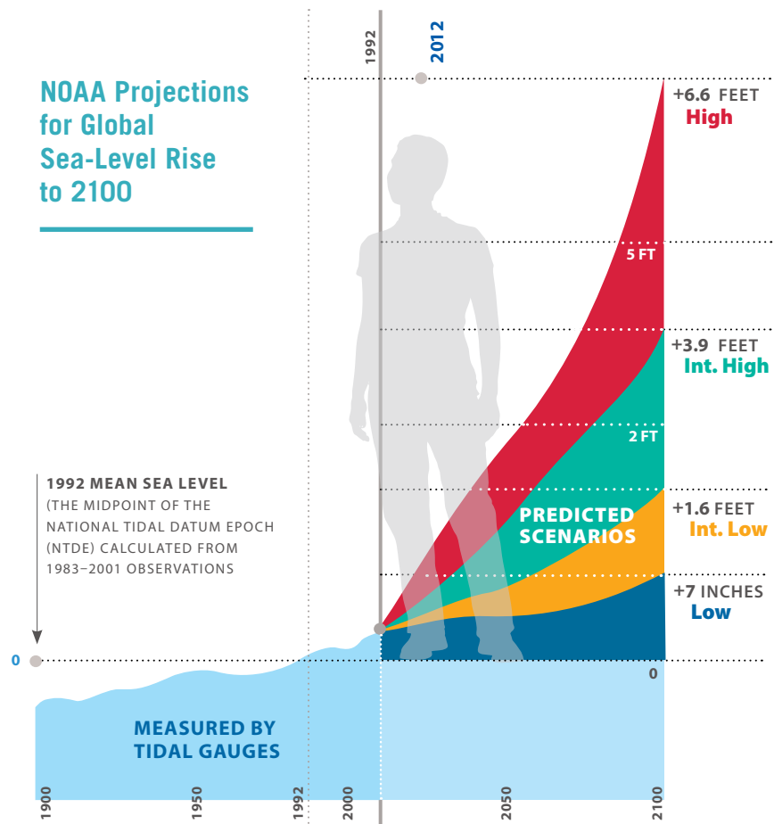
FIGURE 2.9: NOAA PROJECTIONS FOR GLOBAL SEA-LEVEL RISE TO 2100. THE LOWEST SCENARIO ASSUMES VERY MODERATE GLOBAL CLIMATE CHANGE AND A GENERAL CONTINUATION OF THE SEA-LEVEL RISE TREND OBSERVED IN THE 20TH CENTURY TIDE GAUGE RECORD. THE HIGHEST SCENARIO ASSUMES SIGNIFICANT GLOBAL CLIMATE CHANGE THAT INDUCES LARGE-SCALE MELTING OF THE GREENLAND AND ANTARCTIC ICE SHEETS.
