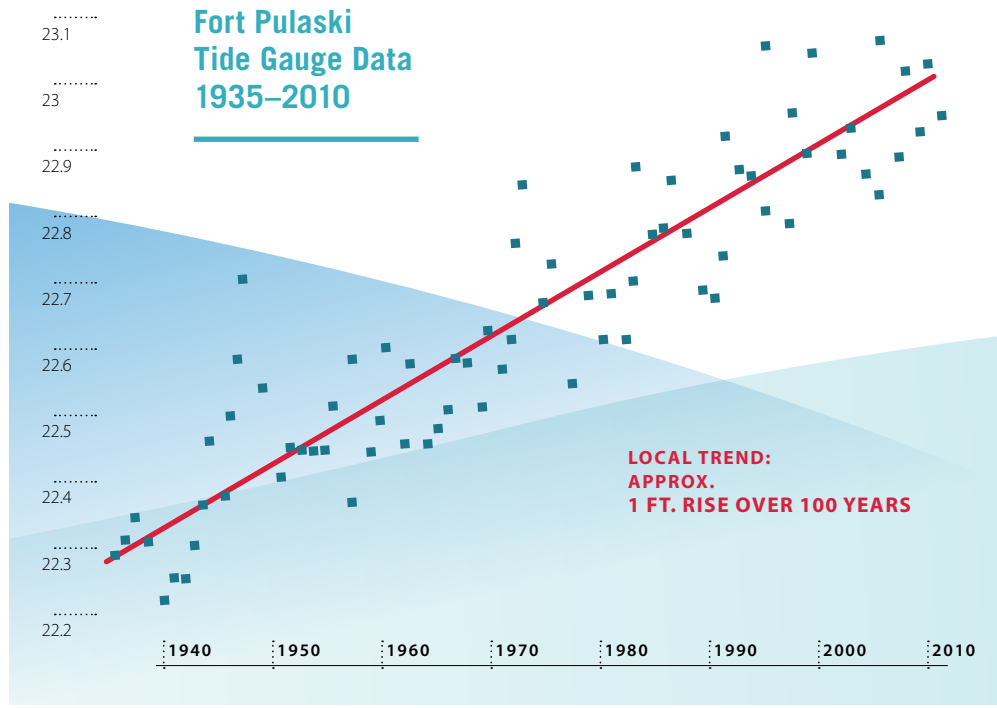
FIGURE 2.8: THE NOAA TIDE GAUGE AT FORT PULASKI HAS RECORDED APPROXIMATELY 10 INCHES OF SEA-LEVEL RISE SINCE 1935.
