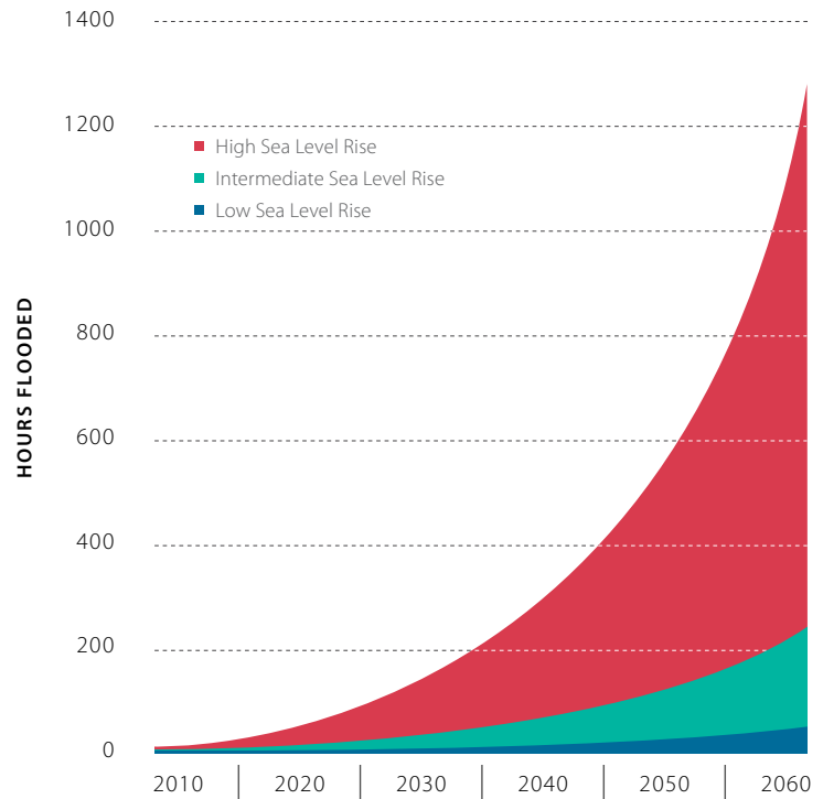
FIGURE 4.4: ANNUAL US 80 TIDAL FLOODING HOURS WITH SEA LEVEL RISE SCENARIOS
