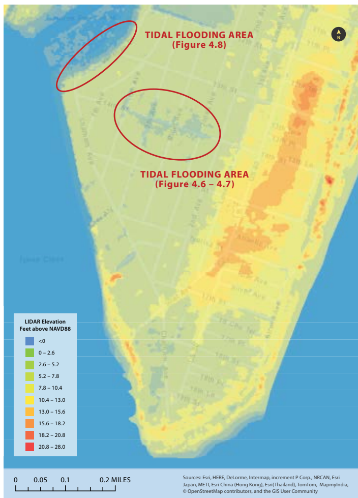
FIGURE 4.5: LIDAR ELEVATION PROFILE FOR CITY OF TYBEE ISLAND, SOUTHWEST QUADRANT
